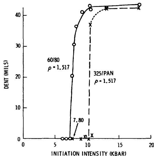
Fig 4 Output of RDX particle sizes (60/80 and 325/pan)
